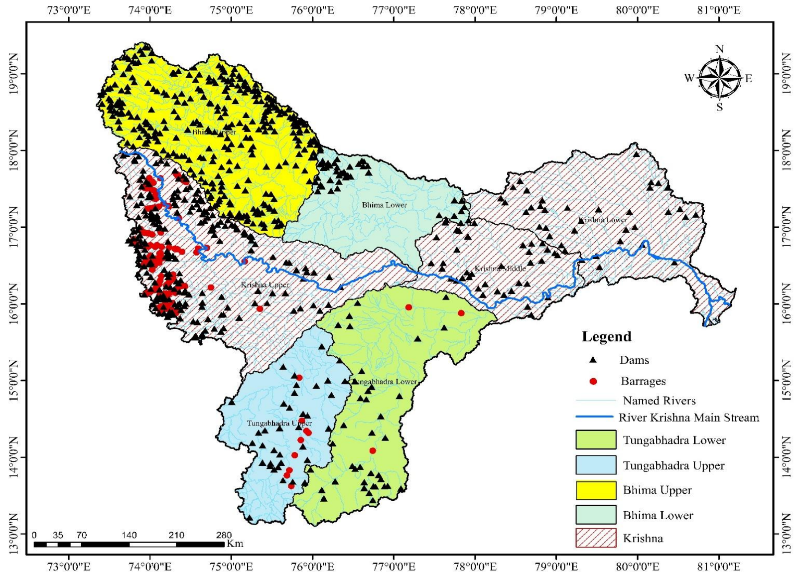
Source: NRLD and WRIS Figure 8: Dams and Barrages in Krishna River Basin
