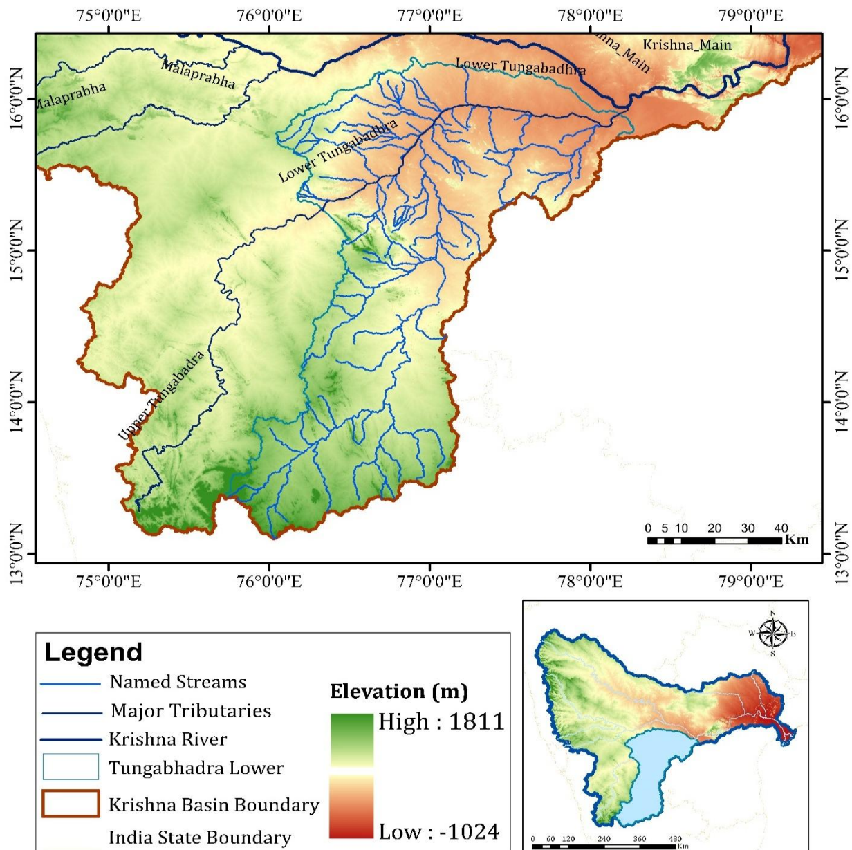
Figure 24: Lower Tungabhadra Basin and it's River Network
