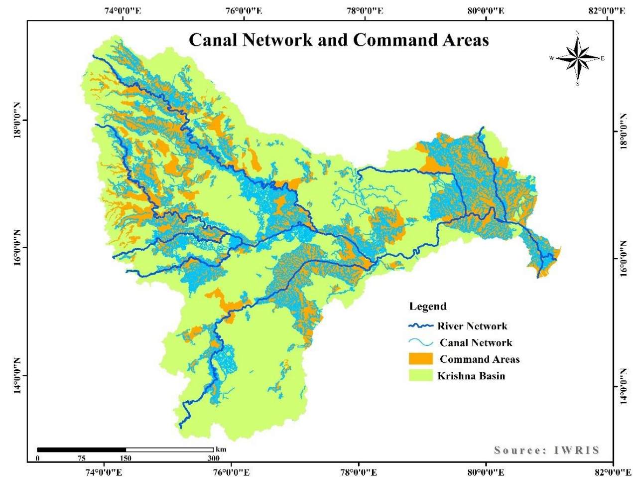
Figure 6: Command Areas and Canal Network in Krishna River Basin
