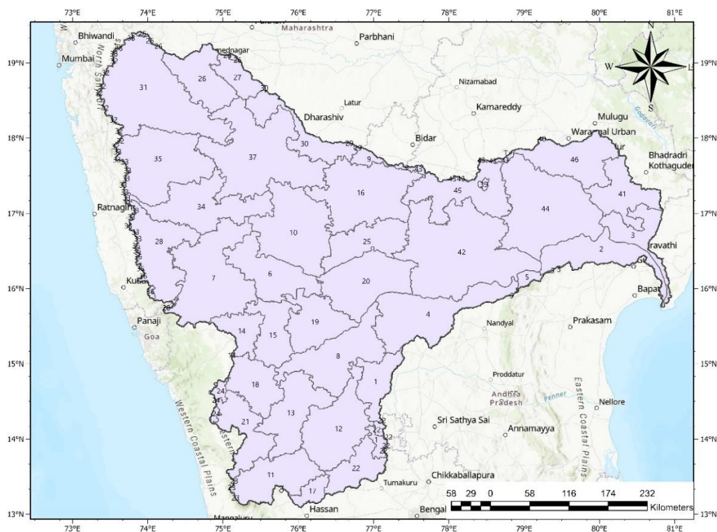
Fig. 13. Districts under Krishna River Basin
