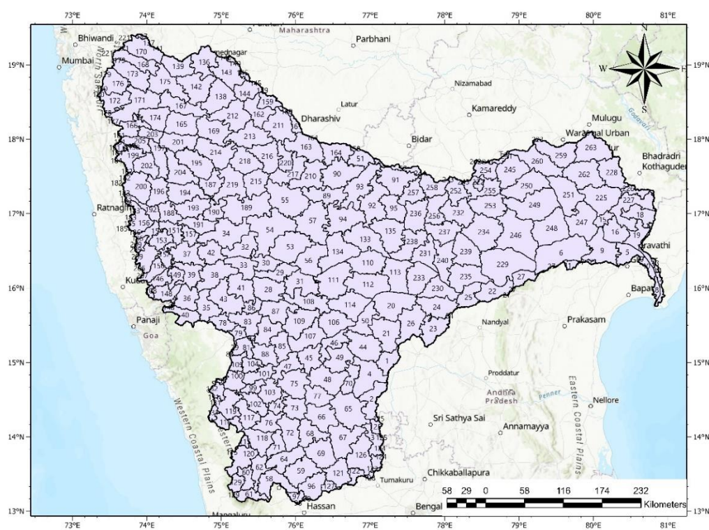
Fig. 14. Taluks (administrative subdivisions) under Krishna River Basin
